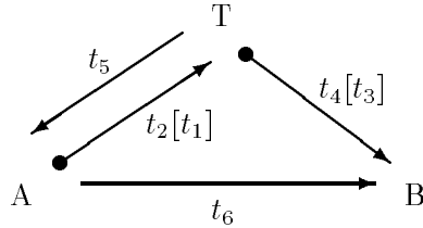
Figure 1. Connecting two authenticated channels by a trusted party T .
