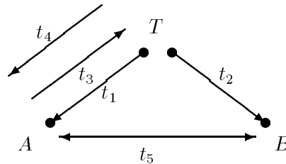
Figure 3. Session key distribution by a trusted server T .
